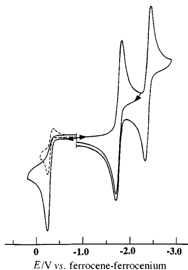
Fig. 2 Cyclic voltammogram of 10^{-3} M [\text{Pt}(\text{bpy})(4\text{-Me}_2\text{NC}_6\text{H}_4\text{S})_2] . Conditions: 10^{-3} M solution in \text{thf}-3 \times 10^{-1} M \text{NBu}_4\text{PF}_6 , 293 K, platinum-disc electrode ( 0.49 \text{ mm}^2 apparent surface area), \nu = 100 \text{ mV s}^{-1} . The dotted curve corresponds to the anodic scan at 210 K
