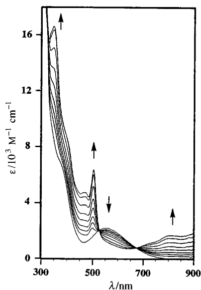
Fig. 3 The UV/VIS spectral changes accompanying the 1e reduction of [\text{Pt}(\text{bpy})(4\text{-Me}_2\text{NC}_6\text{H}_4\text{S})_2] . Conditions: 2 \times 10^{-3} M solution in \text{thf}-3 \times 10^{-1} M \text{NBu}_4\text{PF}_6 , 293 K; electrolysis within an OTTLE cell 10
